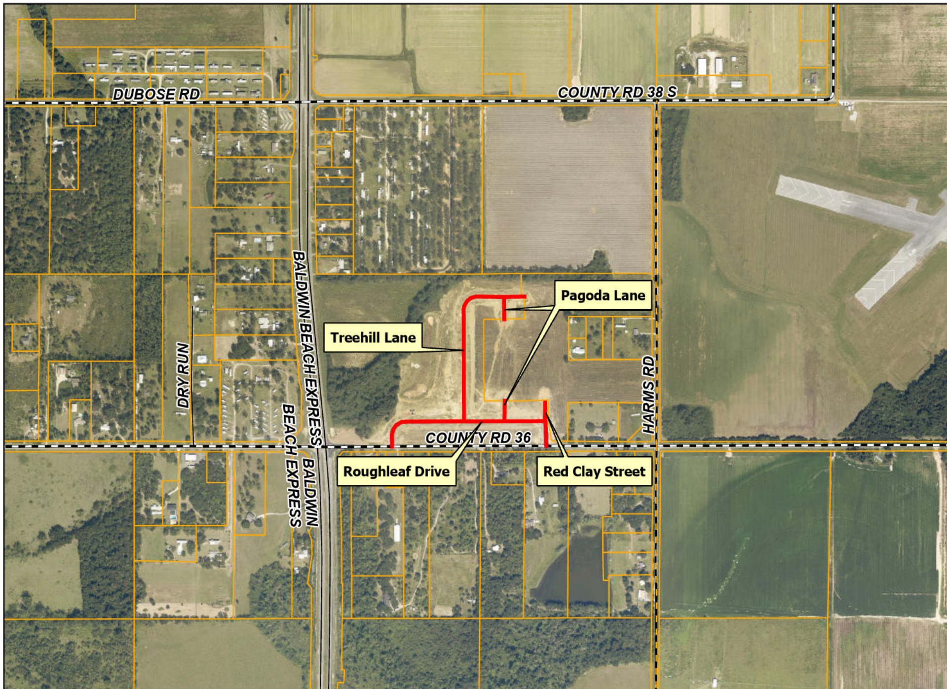
S-21067 Dogwood Estates, Phase 1 Site Map
