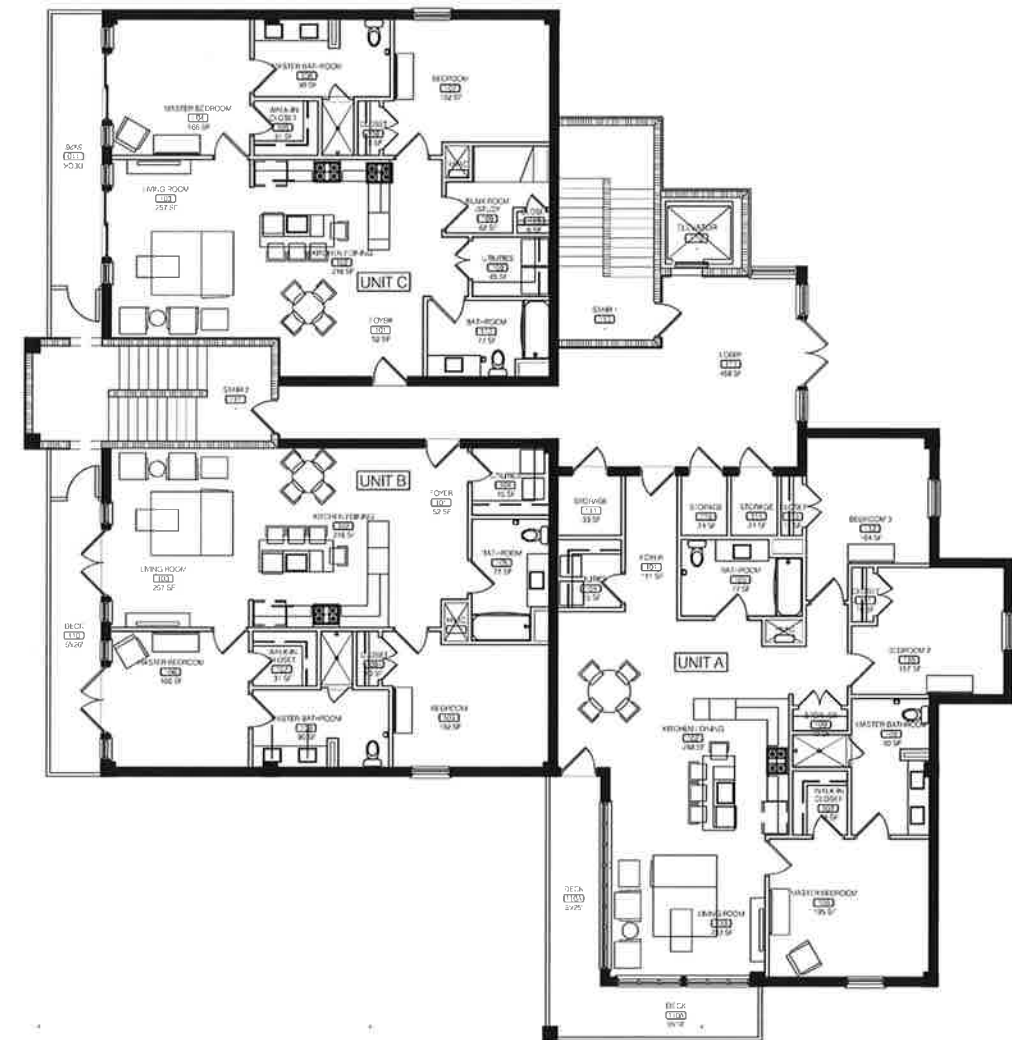
SECOND thru FIFTH LEVEL PLAN SCALE: 1/8" = 1'-0"
