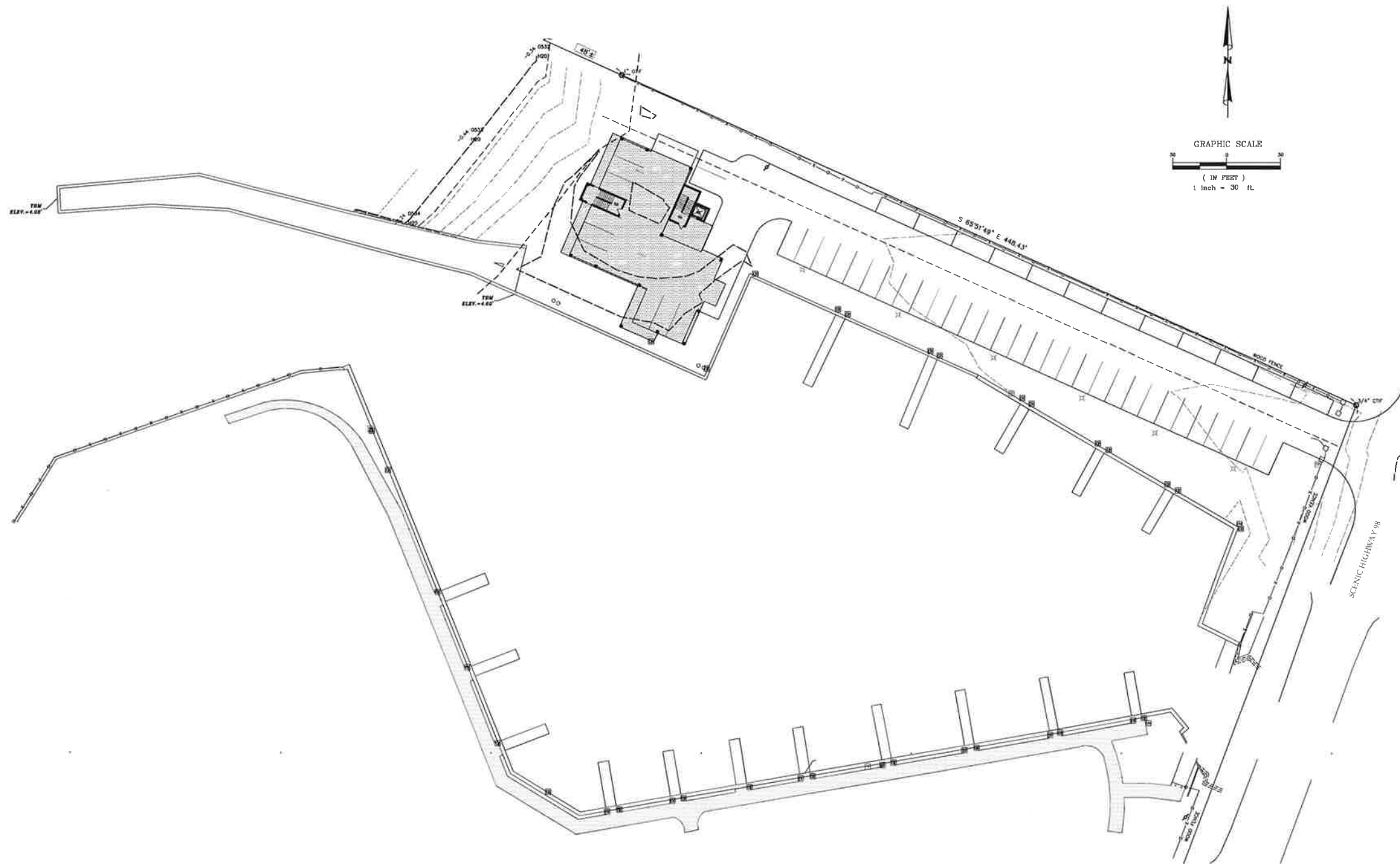
SITE PLAN SCALE: 1" = 30'
