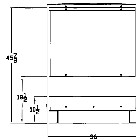
RADIATOR END VIEW
